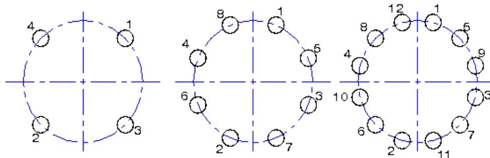
Bolt Tightening Sequence
