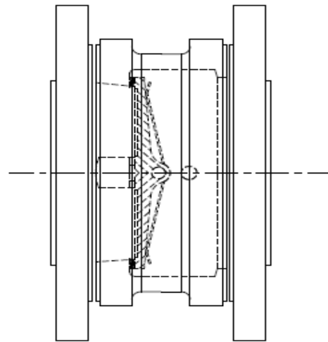
CORRECT INSTALLATION
